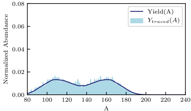
FIG. 7: Comparison of fission yield (solid line) to final traced abundances (shaded region) for the \beta^- -delayed fission of berkelium-270, as in Fig. 6. Nuclei produced by this fission process primarily undergo a series of \beta^- -decays, with minimal effect on the distribution in mass number, A , compared to that of the original yield.
