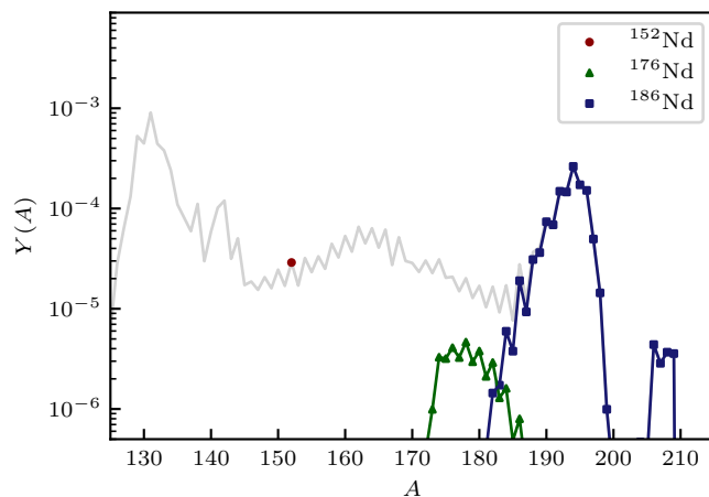
FIG. 9: Traced isotopic abundances for the \beta^- -decay of a selection of neodymium isotopes (neodymium-152, red circle; neodymium-176, green triangles; and neodymium-186, blue squares). The total abundances are given by the gray line for comparison. Neodymium-152 is populated as nuclei are decaying to stable nuclei, and the entirety of abundances for A = 152 have undergone this \beta^- -decay. Neodymium-186 lies on the r -process path, and all nuclei with A \geq 186 have undergone this \beta^- -decay. Neodymium-176 represents an intermediate case, where some fraction, \sim 10\% , of nuclei with A \sim 176 having been produced by this \beta^- -decay.
