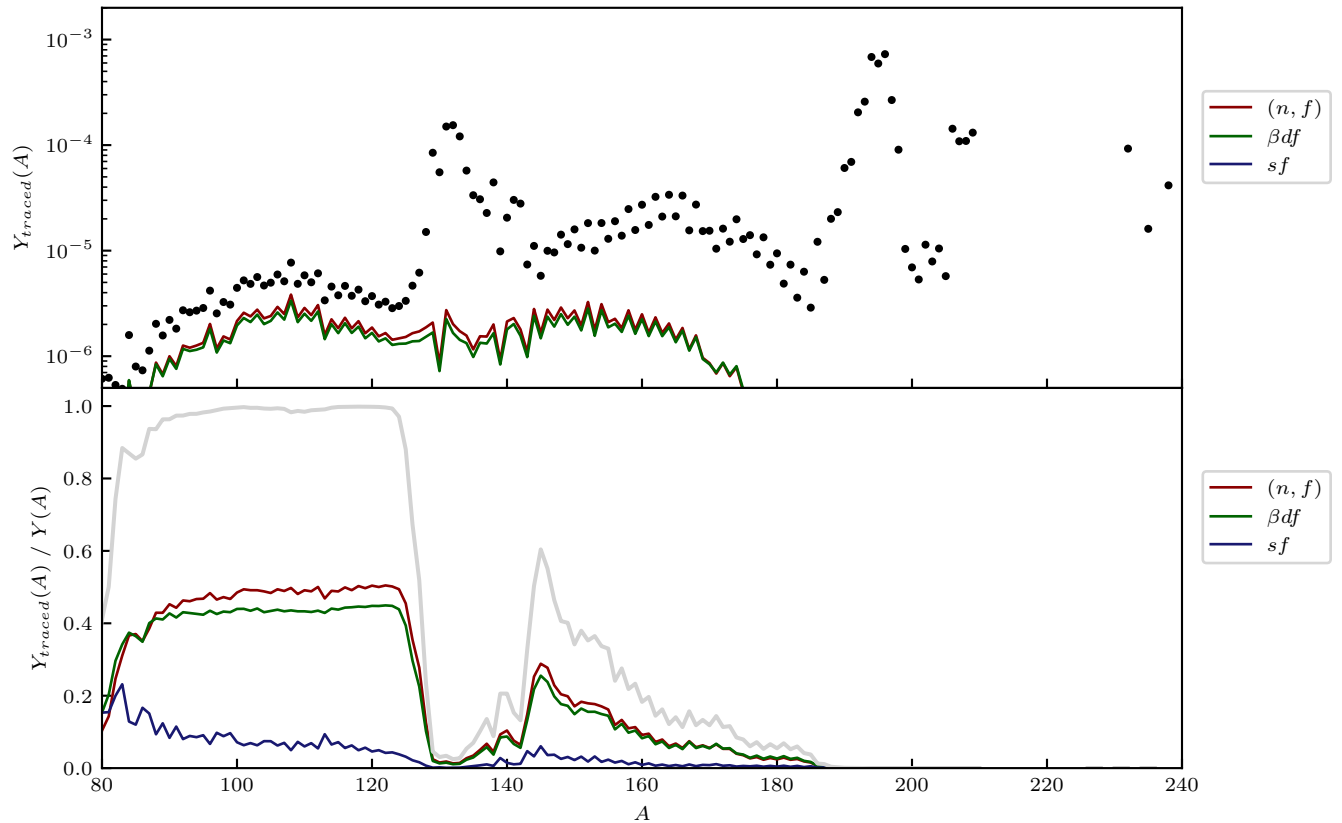
FIG. 2: Relative contributions to final isotopic abundances by terminating fission channel (spontaneous fission, sf ; neutron-induced fission, (n, f) ; and \beta^- -delayed fission, \beta df ) for the neutron star merger wind conditions described in the text. The top panel compares the traced abundances (solid lines) to the total abundances (dots). The bottom panel shows the ratio of each traced abundance to the total abundance; the gray line indicates their sum. For A < 125 , all abundances are populated almost exclusively by fission processes, while the relative contributions to A > 125 are comparatively weaker, peaking at \sim 50\% .
