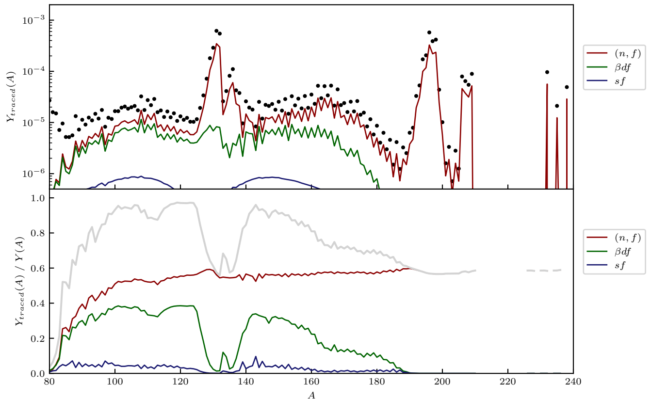
FIG. 3: Relative contributions to final isotopic abundances by terminating fission channel (spontaneous fission, sf ; neutron-induced fission, (n, f) ; and \beta^- -delayed fission, \beta df ) for dynamical ejecta conditions from a neutron star merger simulation [53], as in Fig. 2. For these conditions, nucleosynthesis proceeds via incomplete fission recycling, with neutron-induced fission accounting for \sim 60\% of abundances across the entire range of the pattern, and \beta^- -delayed fission accounting for an additional 10% to 30% for A \lesssim 180 . The remaining abundances, about 10% to 40% depending on A , have no history of fission.
