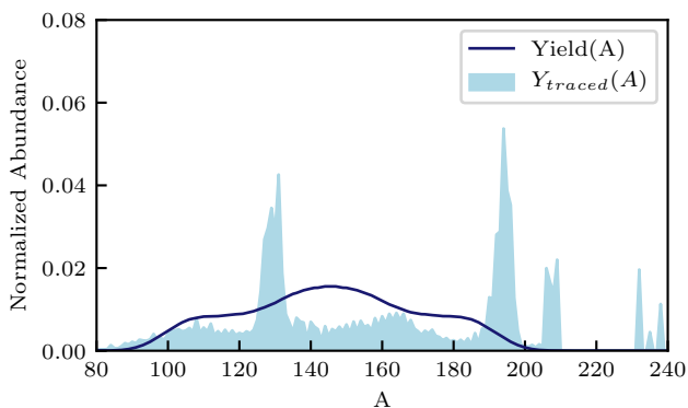
FIG. 6: Comparison of fission yield (solid line) to final traced abundances (shaded region) for the neutron-induced fission of neptunium-290 in the cold dynamical ejecta conditions of [53], as in Fig. 4. Both are normalized according to Eq. 11. Nuclei produced by this fission process participate in significant further neutron-capture nucleosynthesis, with the actual fission yield leaving a minimal imprint on the final abundance pattern.
