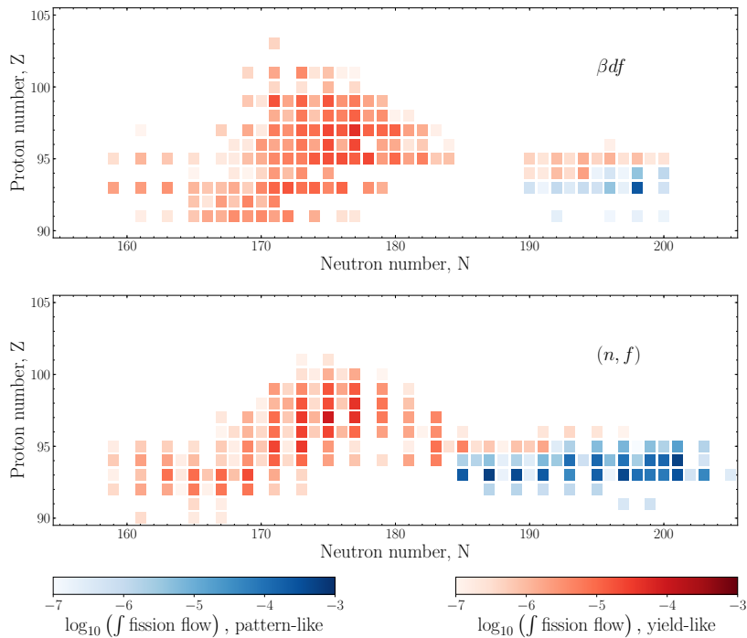
FIG. 8: Integrated \beta -delayed ( \beta df , top panel) and neutron-induced ( (n, f) , bottom panel) fission flows for individual nuclides during the cold dynamical ejecta conditions of [53], as in Fig. 4. Red color indicates that the traced isotopic abundances are mostly similar to the fission yield ( Y_{traced}(A) \sim \text{Yield}(A) , as in Fig. 7), and blue color indicates that the traced isotopic abundances are similar to the overall pattern ( Y_{traced}(A) \sim Y(A) , as in Fig. 6).
