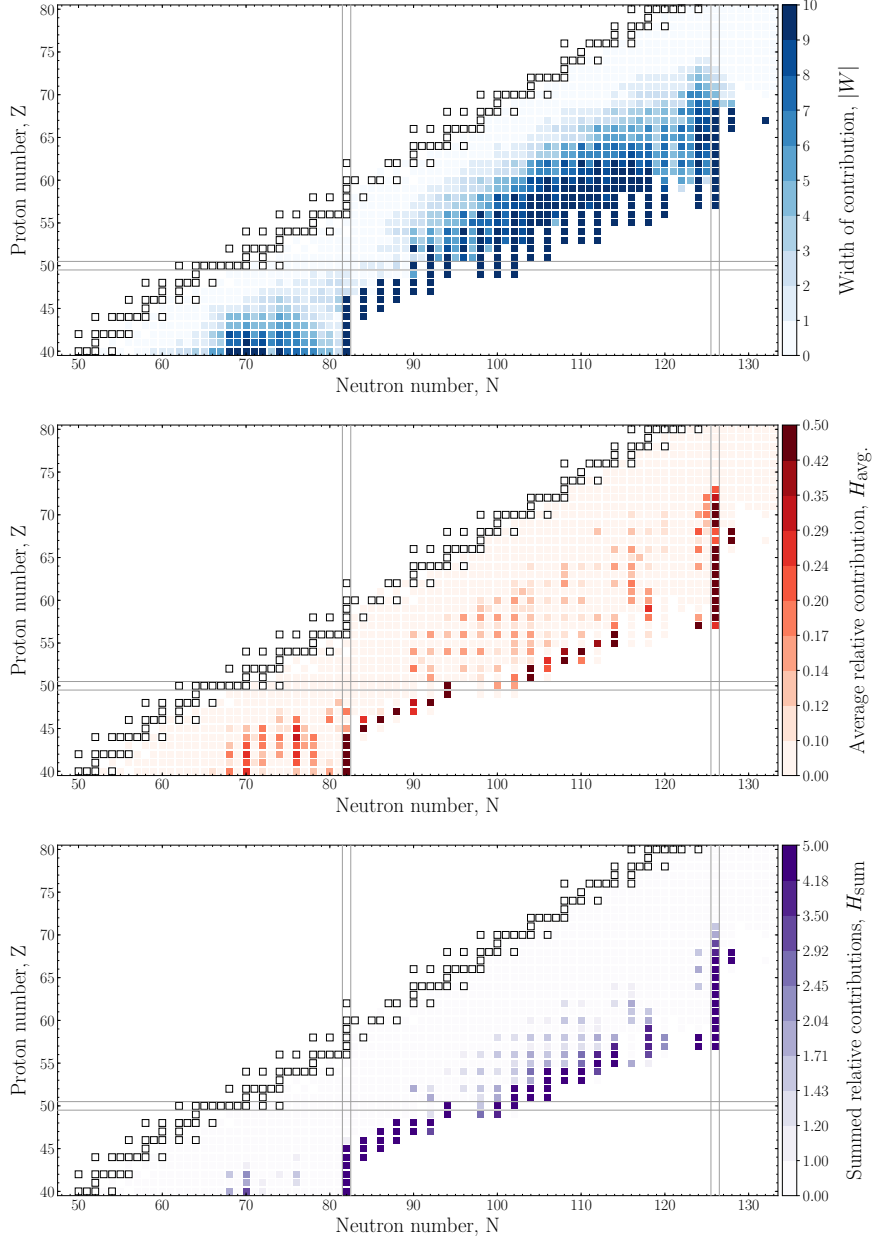
FIG. 10: Average trends in the traced abundances of individual \beta^- -decays for elements 40 < Z < 80 . The top panel shows the ‘width’ ( |W| ) of the traced abundances, as defined in the text. The middle panel indicates the average relative contribution to total abundances contained within the width ( H_{\text{avg}} ). The bottom panel gives the the sum of relative contributions to the width ( H_{\text{sum}} ), which may be interpreted as the product of the top and middle panels.
