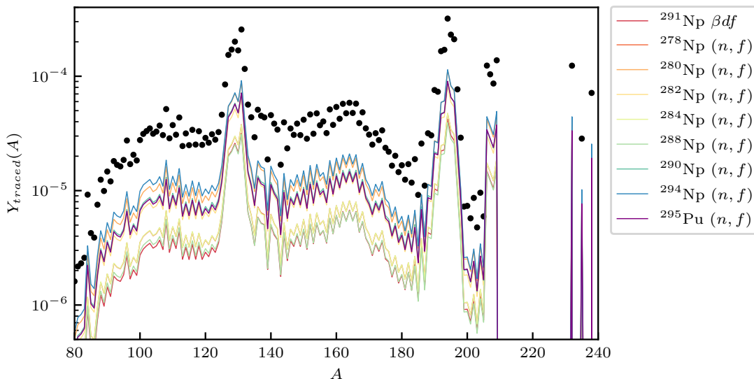
FIG. 5: Relative contributions to final isotopic abundances, Y(A) , solid dots) for the \beta^- -delayed ( \beta df ) and neutron-induced ( (n, f) ) fission products of individual neptunium and plutonium isotopes (solid lines) in the cold dynamical ejecta conditions of [53], as in Fig. 4. The plotted isotopes are those whose fission yields contribute at least 10% to the total abundance pattern for at least one mass number A .
