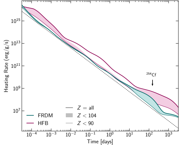
Figure 2. Heating rates over time for two extremes of nuclear variations showing the contribution by all elements (thick, solid lines), only up to the actinides (shaded), and excluding the actinides and superheavy elements (thin, solid lines). The dashed line is a simple model in which the heating rate evolves scales with time by 10^{-1.3} (see, e.g., Metzger 2019 ). The divergence between the shaded region and the thick lines (e.g., at about 10^{-2} – 10^1 days for HFB) indicates heating uniquely from the superheavy elements.
