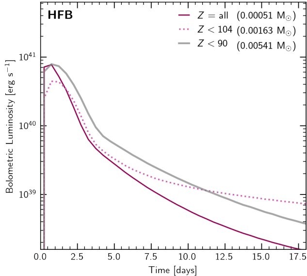
Figure 4. Bolometric light curves for the HFB model (right) with ejecta es renormalized such that the heating rates at one day is equal for all models. Three sets of heating rates: only Z < 90 elements (gray), only Z < 104 elements (dashed pink), and all elements (dark pink).
